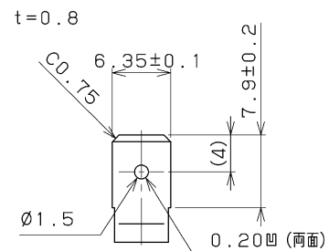
端子部詳細 (2:1)
